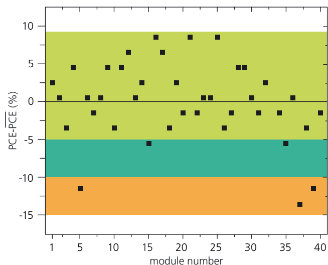
Graph: Deviation of the power conversion efficiency from the mean value determined from measurements of 39 modules.
